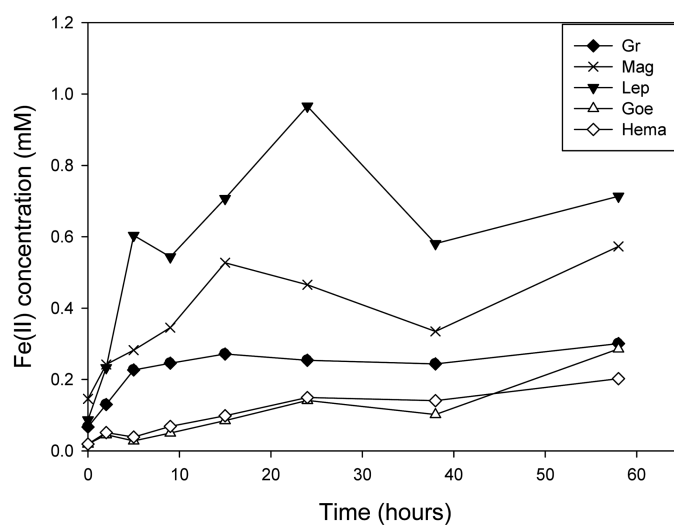
Fig. 8 Production of 3N HCl extractable Fe(II) during the reductive degradation of RDX by interaction of bio-reduced IBSMs (green rust, magnetite, lepidocrocite, goethite, hematite) (0.1 g/200 mL) and CN32 in MDM at pH 7 (PIPES)
