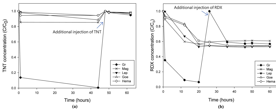
Fig. 1 Abiotic reductive degradations of (a) TNT and (b) RDX by IBSMs (green rust, magnetite, lepidocrocite, goethite, and hematite) (0.1 g/200 mL) in DDW. The initial concentrations of TNT and RDX were 0.22 and 0.05 mM, respectively
