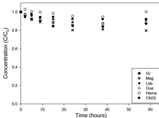
Fig. 2 Enhanced reductive degradation of TNT by bio-reduced IBSMs (green rust, magnetite, lepidocrocite, goethite, and hematite) with CN32 and only CN32 in MDM at pH 7 (PIPES). The initial concentration of TNT was 0.22 mM
