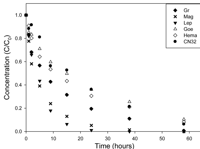
Fig. 7 Enhanced reductive degradation of RDX by bio-reduced IBSMs (green rust, magnetite, lepidocrocite, goethite, and hematite) with CN32 and only CN32 in MDM at pH 7 (PIPES). The initial concentration of RDX was 0.05 mM
