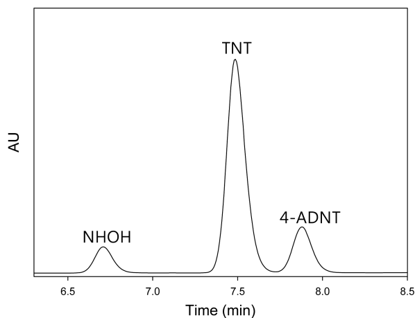
Fig. 6 HPLC chromatogram showing the production of 4-ADNT during the enhanced reductive degradation of TNT by bio-reduced green rust at 38 h
