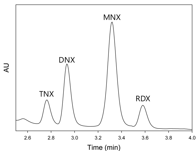
Fig. 9 HPLC chromatogram showing the production of MNX, DNX, and TNX during the enhanced reductive degradation of RDX by bio-reduced green rust at 38 h
