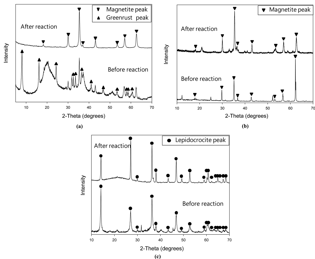
Fig. 4 (a) XRD pattern showing the transformation of green rust to magnetite during the reductive degradation of TNT by bio-reduced green rust, (b) and (c) XRD patterns showing no mineral transformations of magnetite and lepidocrocite during the enhanced reductive degradation of TNT: peaks of green rust (▲), magnetite (▼), and lepidocrocite (●)
