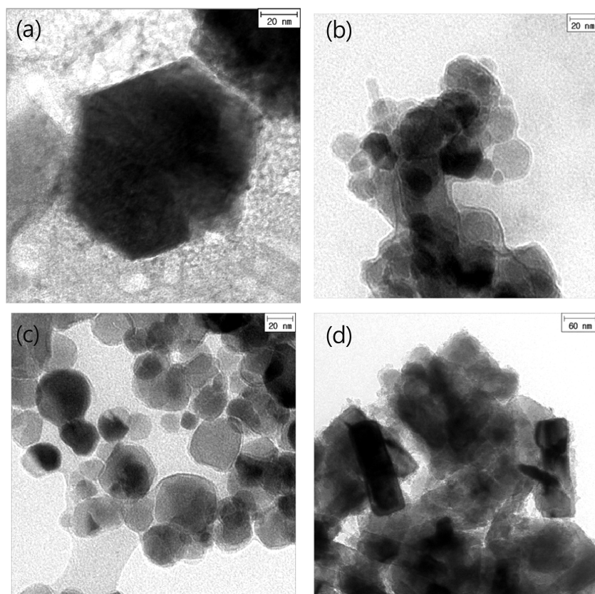
Fig. 5 TEM images of (a) green rust and (b) magnetite before and after the reductive degradation of TNT at 58 h, TEM image of (c) chemogenic magnetite and (d) chemogenic lepidocrocite after the reductive degradation of TNT showing no mineral transformations
